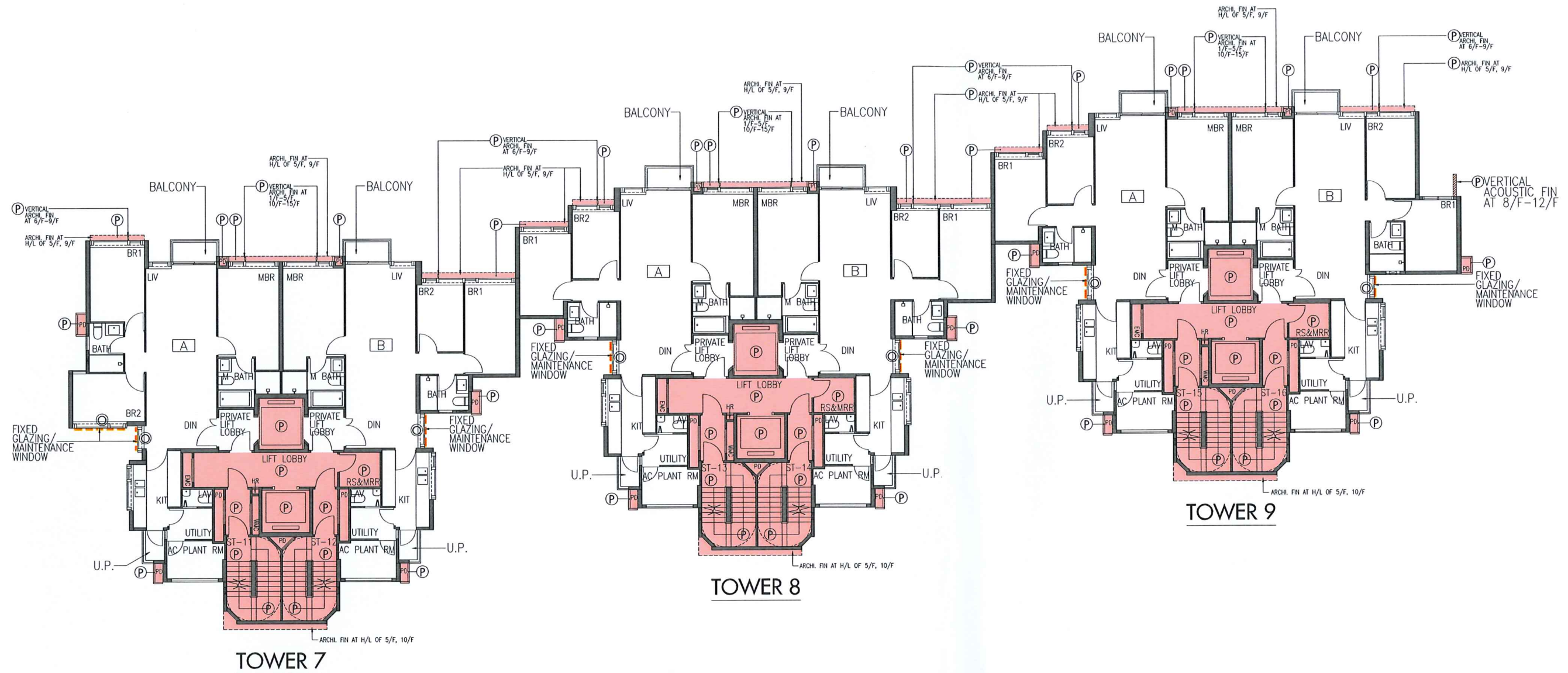
TOWER 7-9 2/F-12/F FLOOR PLAN 1:200 \nearrow (4/F, 13/F, 14/F TO BE OMITTED)
